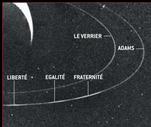
LE VERRIER AND ADAMS RINGS
