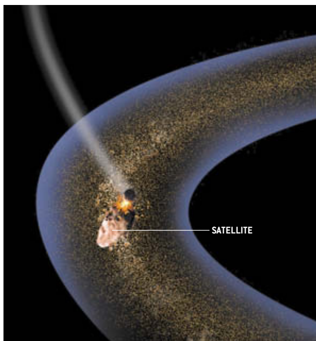
IF SOMETHING SLAMS into a satellite, material flies off and becomes part of a ring. Conversely, the satellite steadily sweeps up material. The balance of these competing effects determines the size of faint rings.
